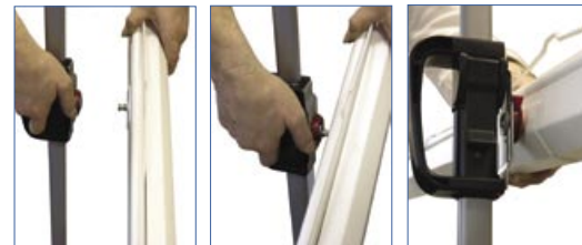
Tension device - adjusts bottom picture level / locks screen in any format.
