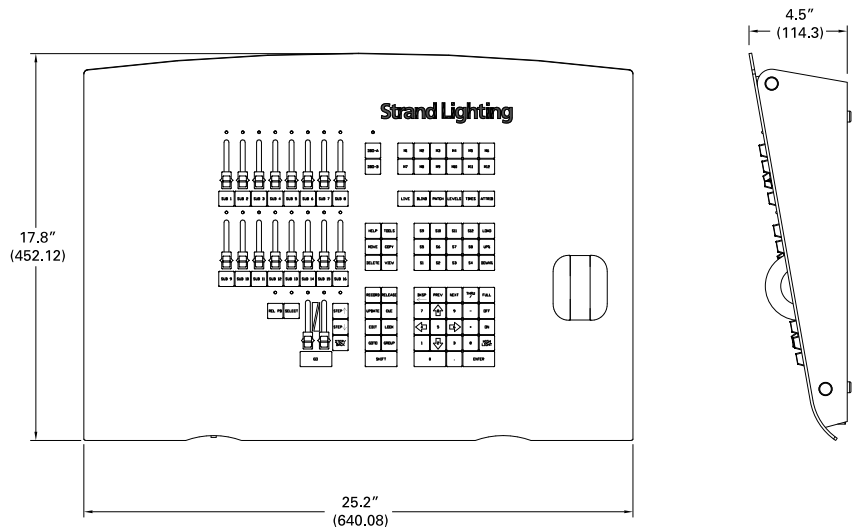
91800 classicPalette Basic Memory Console with 100 channels, 16 submasters*
