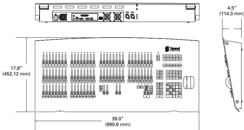
91801 presetPalette Memory-Manual Console 32/84 with 100 channels
