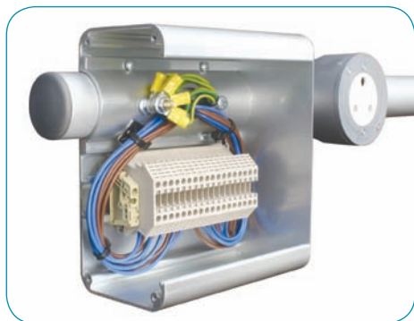
Extruded Side Mounted Terminal Box
